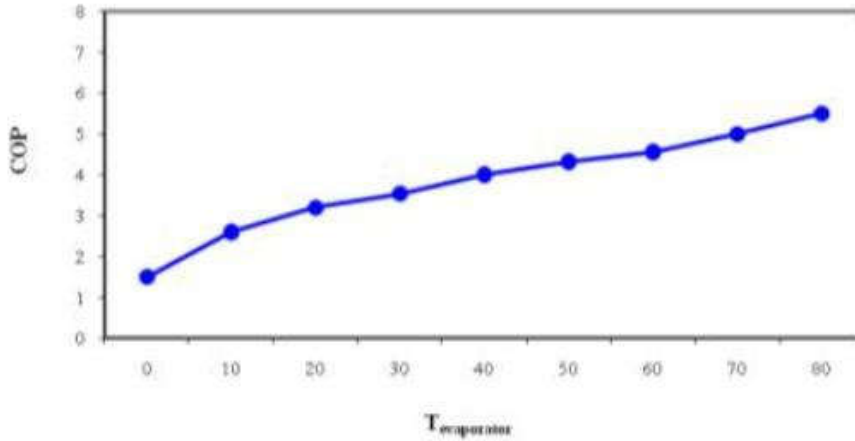
Figure 6. Heat pump performance vs evaporation temperature.
