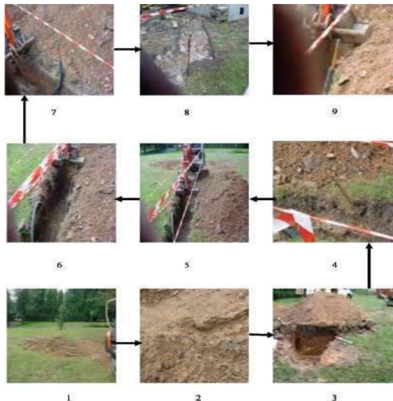
Figure 3. Showing the drilling (1-2) digging of the pit (3), connection of the manifolds (4), grouting, preparation of the coils (5-6) and the source loop, which consists of two earth loops: one for vapour and one for liquid (7-9).
