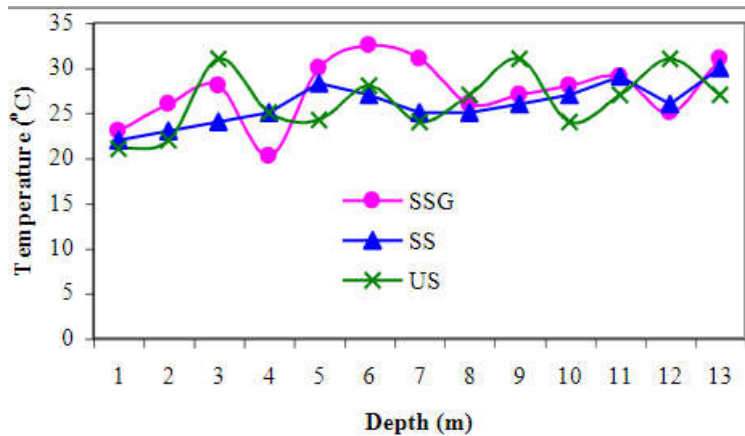
Figure 13. Comparison of experiments for saturated soil with groundwater flow (SSG), saturated soil without groundwater flow (SS) and unsaturated soil without groundwater flow (US).
