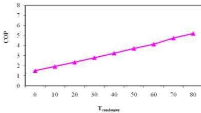
Figure 7. Heat pump performance vs condensation temperature.
