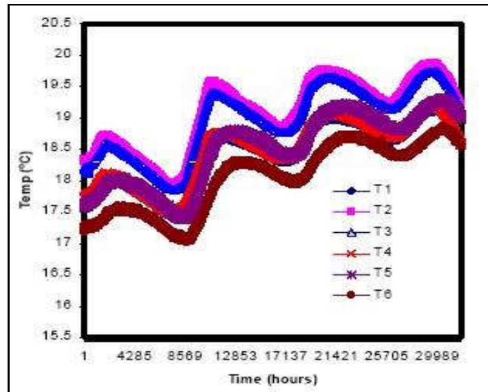
Figure 19. Variation of temperatures for heat exchanger for year.
