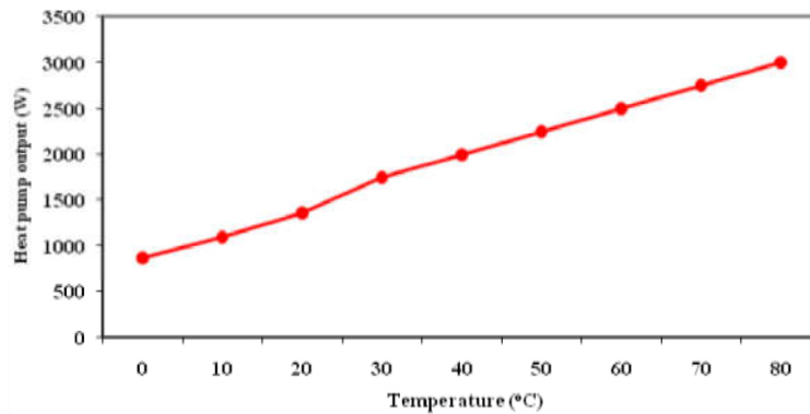
Figure 20. Variation of heat pump output with temperature.
