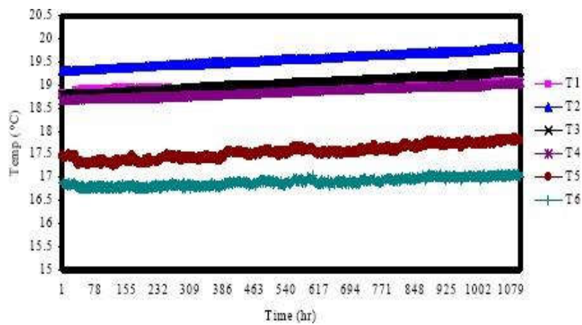
Figure 18. Variation of temperatures for heat exchanger for 45 days.
