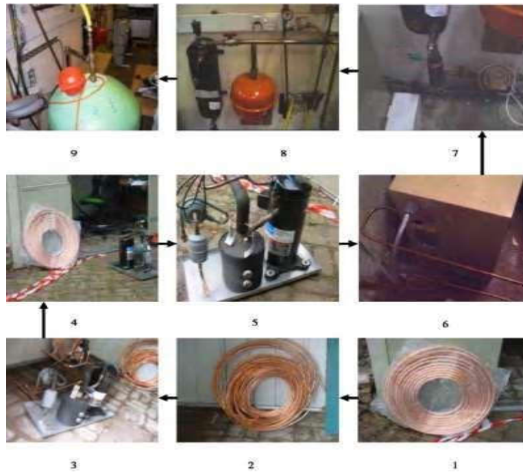
Figure 4. Showing preparation of coils (1-2), installation of heat pump (3-6) and connection of water supply system (water pump, flow metre, expansion valve and the boiler) (7-9).
