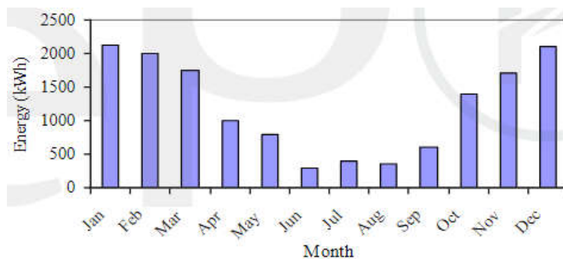
Figure 22. Monthly heating energy demands.
