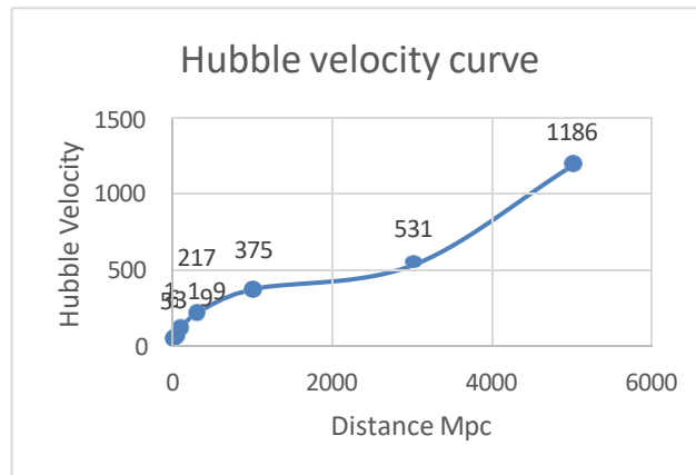
Fig. 5,6 :Hubble velocity(km/sec/Mpca) curve and expansion coefficient( MF=10^{-55} ) as derived by wave theory
