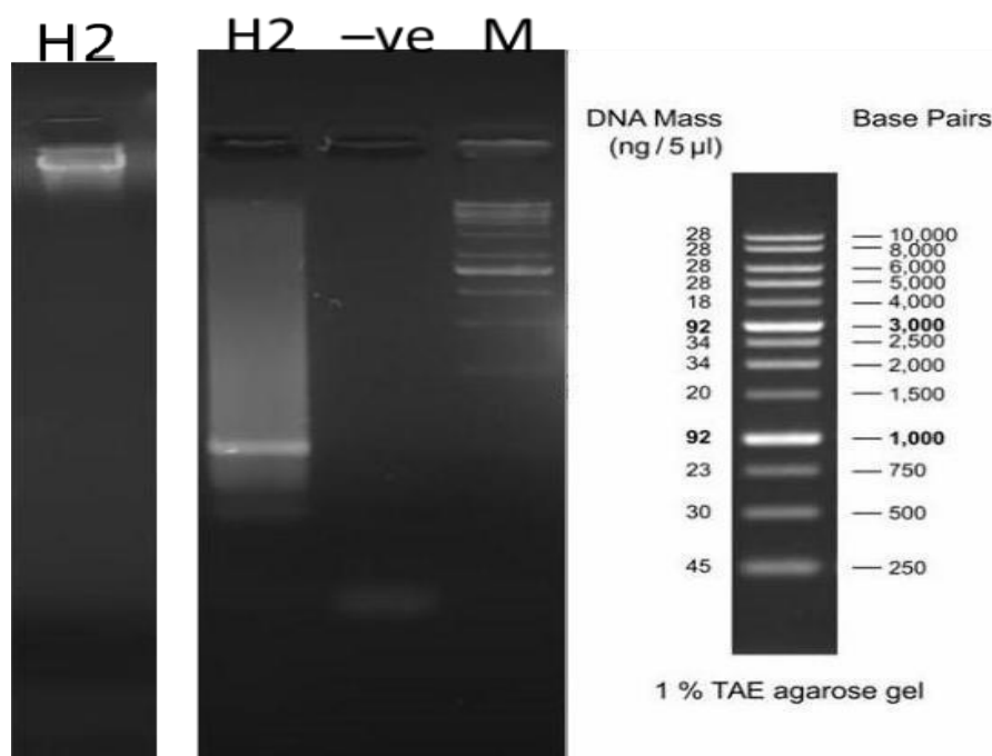
Figure a: Isolated genomic DNA Figure b: Quality check of PCR subjected to 1% agarose gel. Product Subjected to 1.5% Agarose gel electrophoresis. M is 1000 bp marker.
