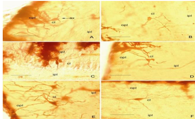
Fig. 6. Photomicrographs showing neurons of the dorsal cerebral cortex of Calotes versicolor : pyramidal neuron (A); monotufted bipolar neuron (B-D); inverted pyramidal neuron (E-F). Scale bar = 50 \mu m.
