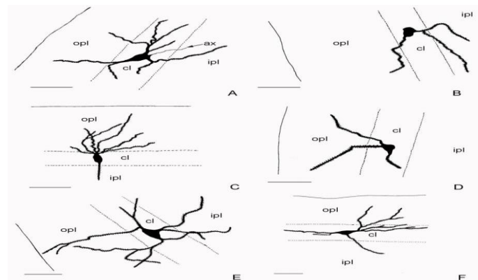
Fig. 7. Camera lucida drawings of the dorsal cerebral cortex neurons of Calotes versicolor : pyramidal neuron (A); monotufted bipolar neuron (B-D); inverted pyramidal neuron (E-F). Scale bar = 50 \mu m.
