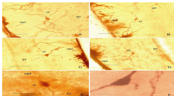
Fig. 8. Photomicrographs showing neurons of the dorsal cerebral cortex of Calotes versicolor : bitufted neuron (A-C); monotufted neuron (D); aspiny bipolar neuron (E-F). Scale bar; A-E = 50 \mu m, F=10 \mu m.
