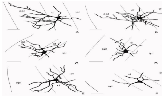
Fig. 5. Camera lucida drawings of the dorsal cerebral cortex neurons of Calotes versicolor : multipolar neurons (A-D); pyramidal neuron (E-F). Scale bar = 50 \mu m.
