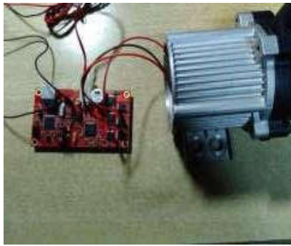
Fig.6 High Integration Sensorless Brushless DC Motor Experimental Platform
