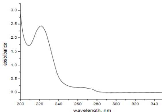
Figure (3): Spectrum of benzoic acid indicate the single UV absorption band at \lambda_{max} = 221 nm.
