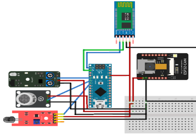
Fig.3- Circuit for the sensor's unit
