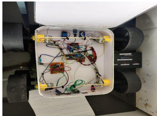
Fig.16- Hardware placement
