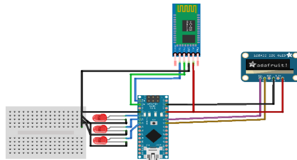
Fig.4- Circuit for the receiving unit
